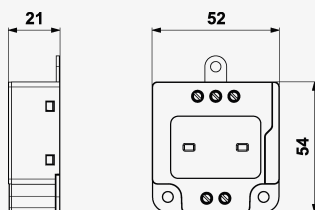
Product dimensions
