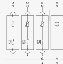
Basic circuit diagram
