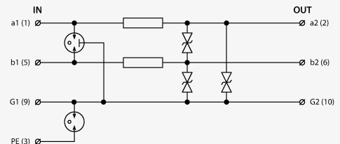
Basic circuit diagram
