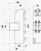
Product dimensions
